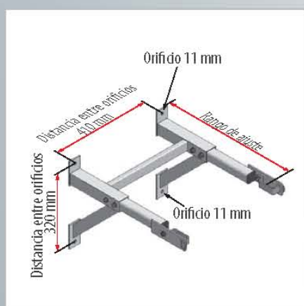
Consola mural, ajustable
