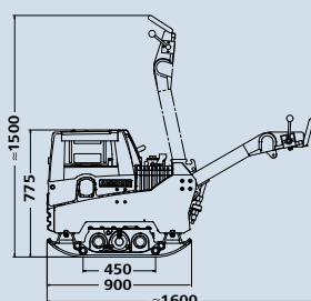
APH 5030
