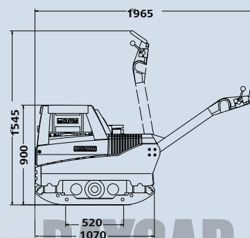
APH 100-20
