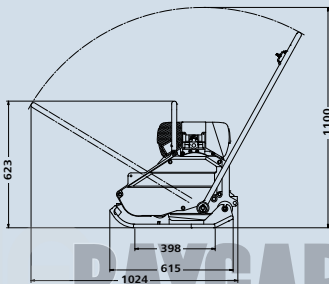
APF 1850 Hatz
