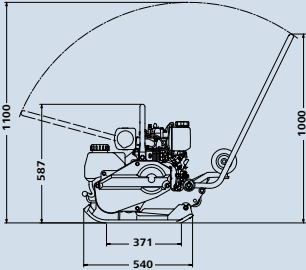
APF 1240 Yanmar
