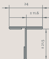
Tapajuntas Fijo Couvre-joints Imposte Fix Joint Cover
