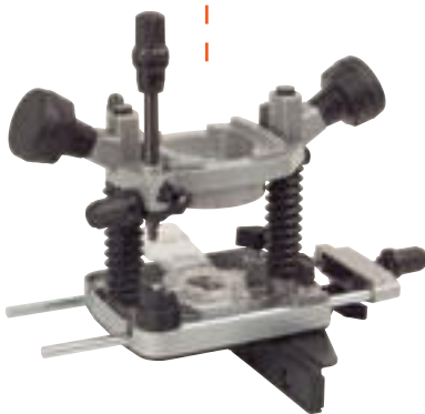
Optional Routing head with lateral fence and fine adjustment. Ref. 5646670
